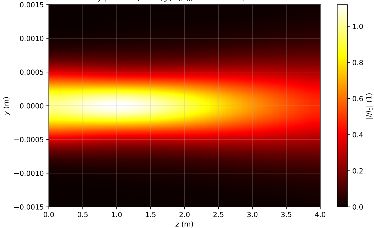
Intensity profile I(x=0, y, z)/I_0 , P_{in}=0.6P_{cr} , artificial time
